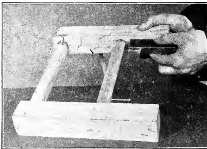
Fig. 220—Testing with Trysquare
